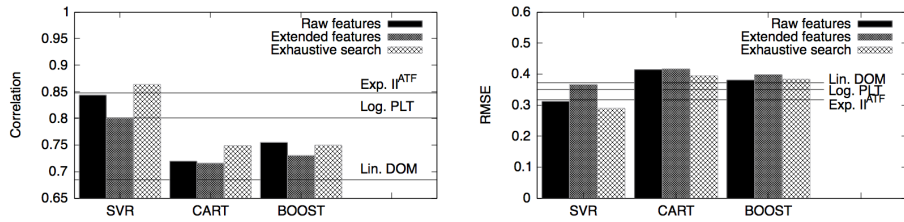
Fig. 4: Machine learning: Comparison of ML algorithm using different feature sets against reference expert models, for (a) correlation and (b) RMSE metrics
