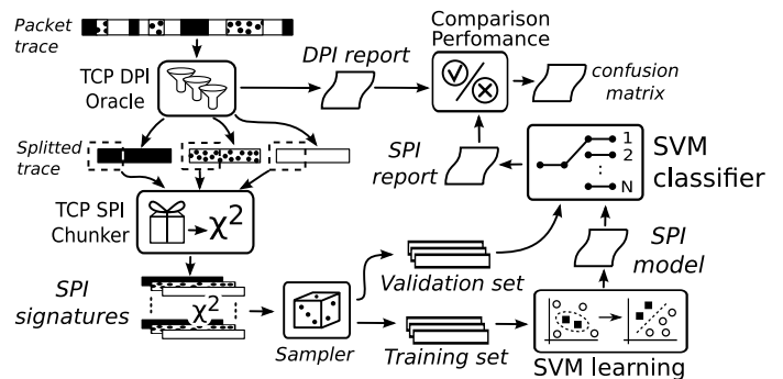
Fig. 3. Classification Workflow
