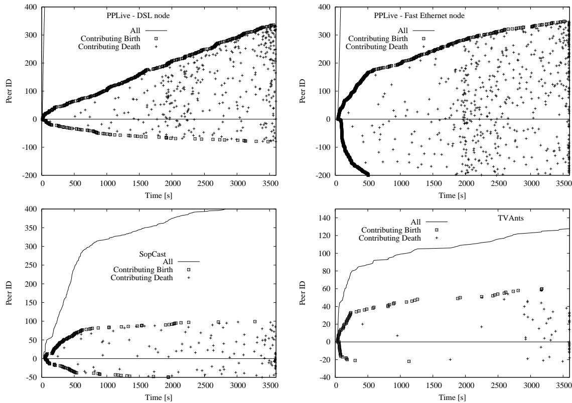
Fig. 4. Arrival and Departure process of the all and video contributing peers.
