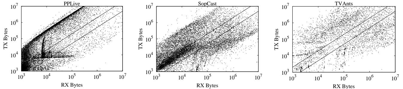
Fig. 3. Scatter plot of RX versus TX bytes, guidelines represent the tit-for-tat boundaries Tx/Rx=2 and Rx/Tx=2
